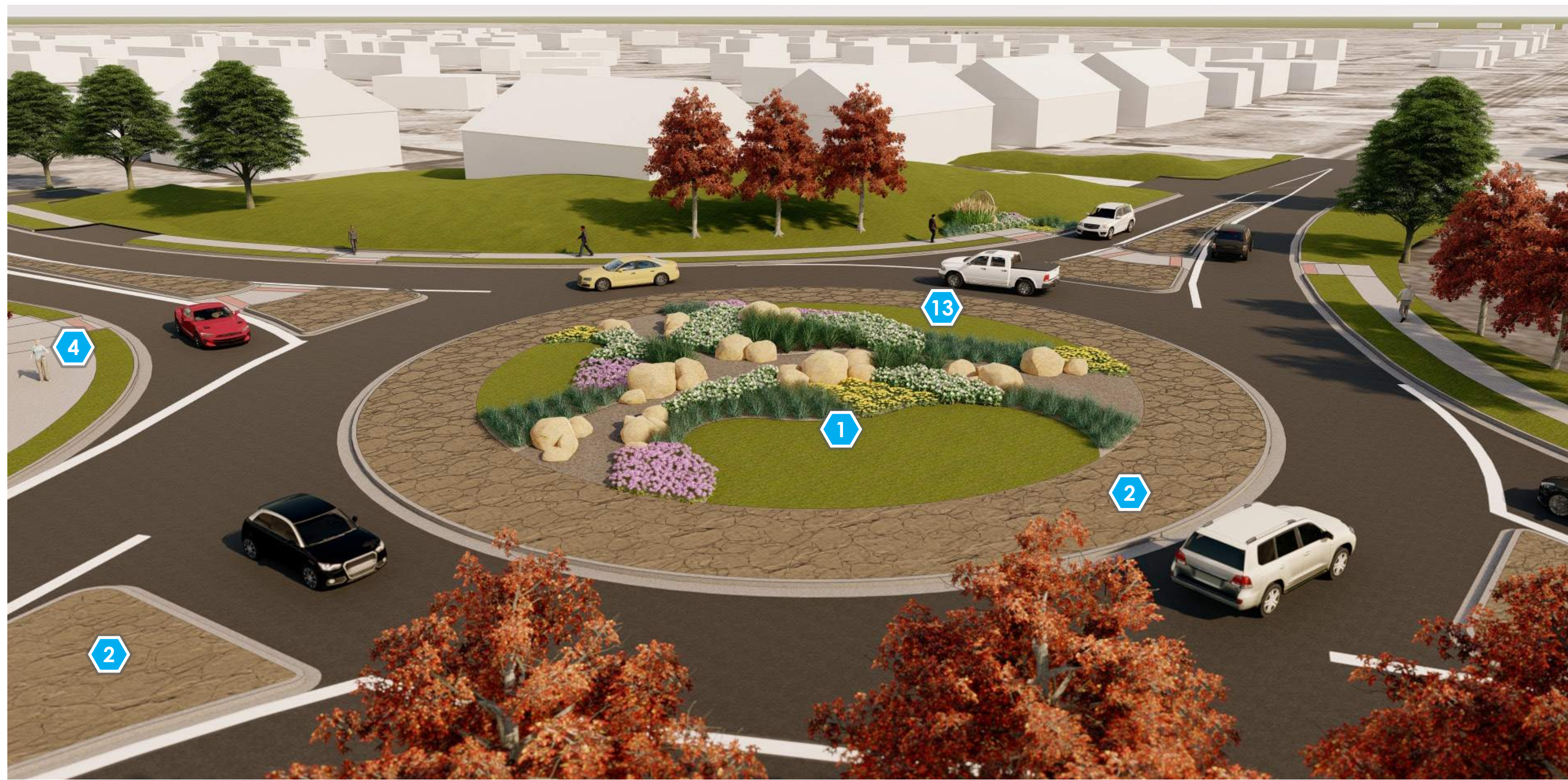
BIRD'S EYE VIEW OF ROUNDABOUT LOOKING EAST ON PARALLEL ROAD
